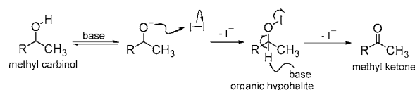
Scheme 3. Oxidation of the Methyl Carbinol to the Methyl Ketone
